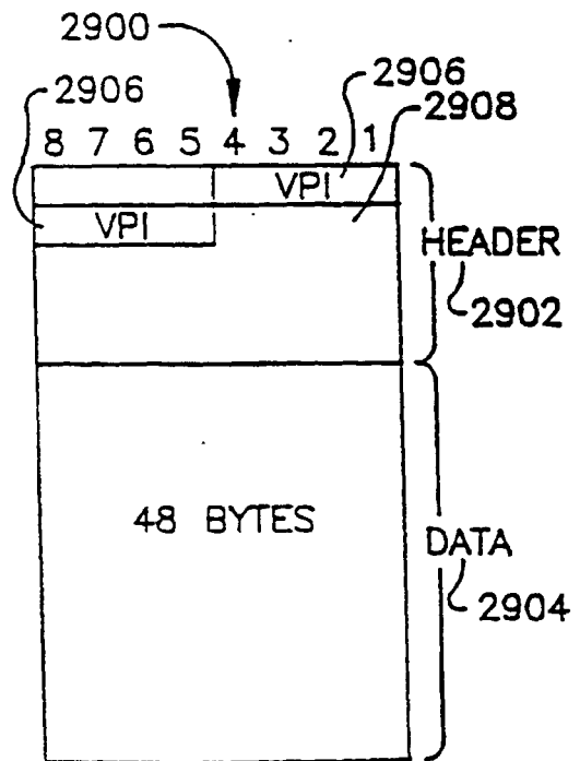
TDM CELL
