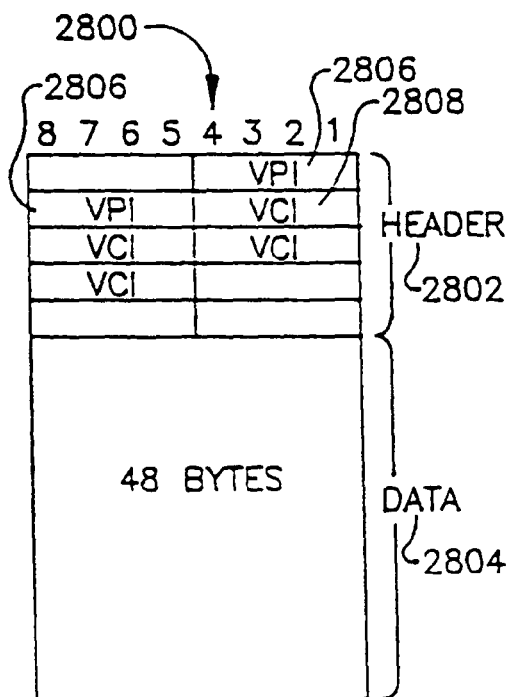
ATM CELL
