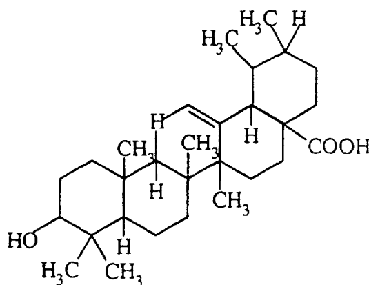
Ursolic Acid
