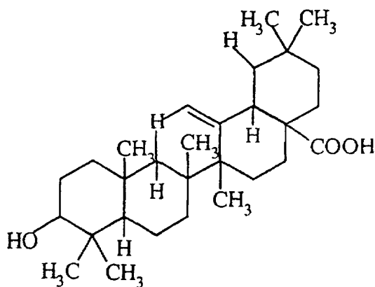
Oleanolic Acid
