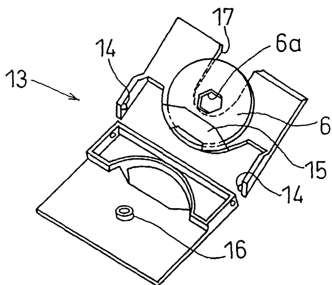
FIG.18 (Prior Art)
