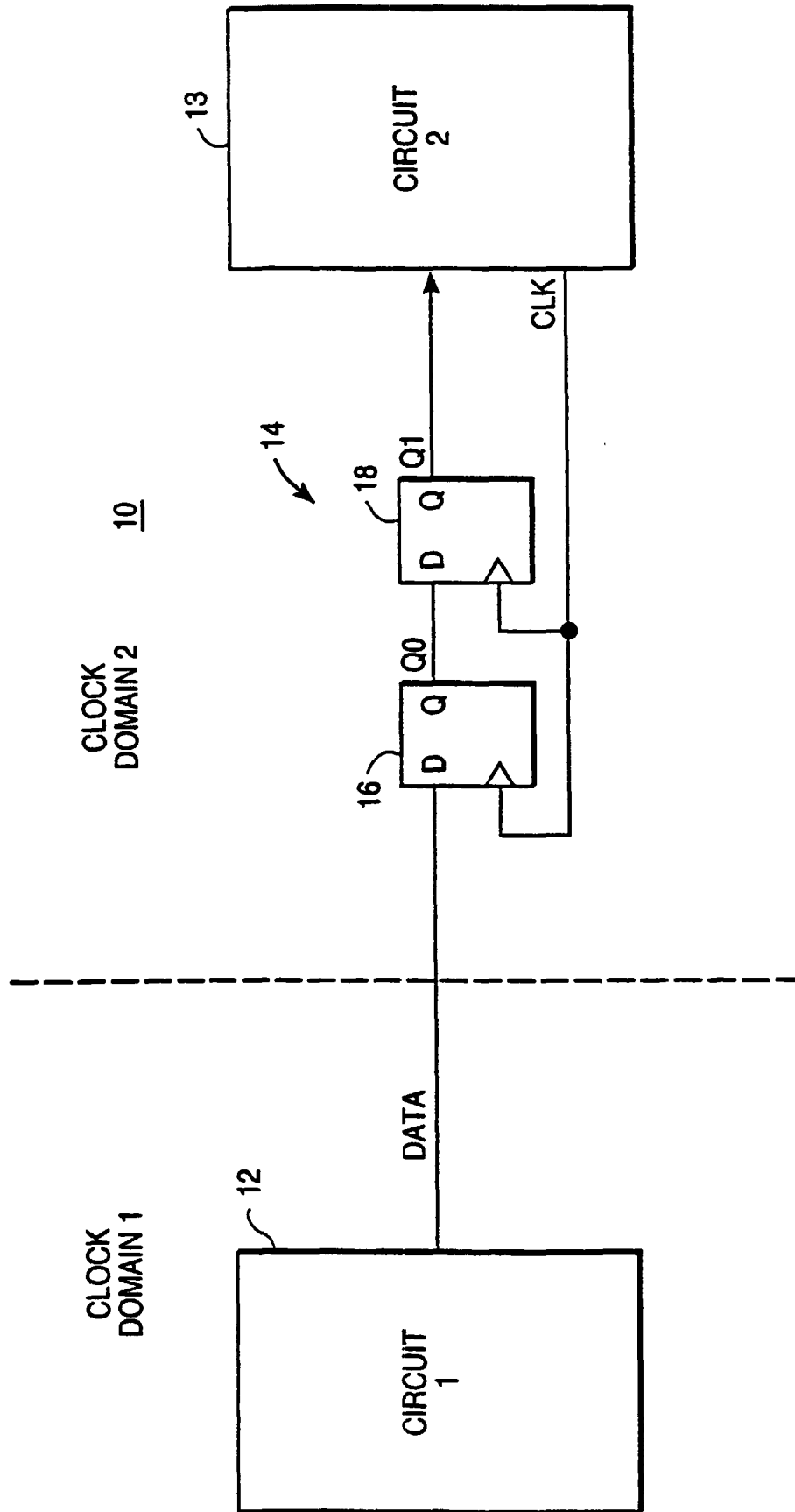
FIG. 1 (PRIOR ART)
