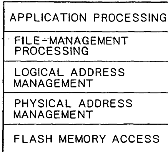
PROCESSING HIERARCHY OF A FILE SYSTEM
