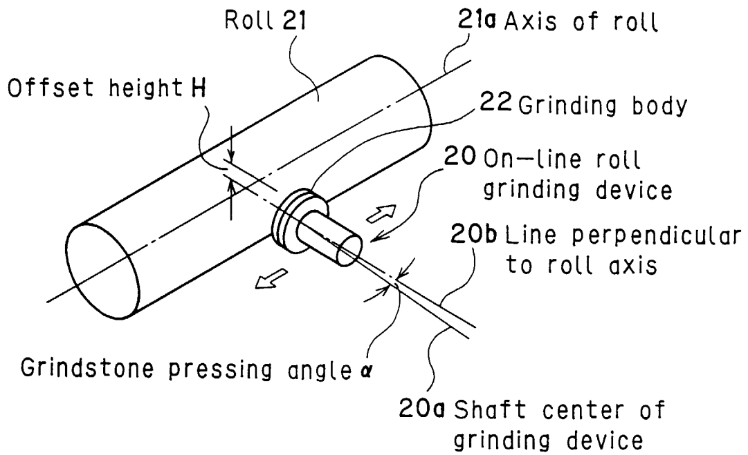
Fig.16 Related Art
