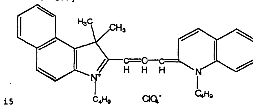
[Chemical Formula 239]
