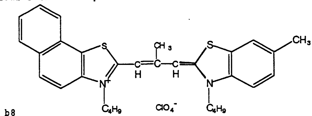
[Chemical Formula 206]
