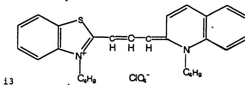
[Chemical Formula 237]
