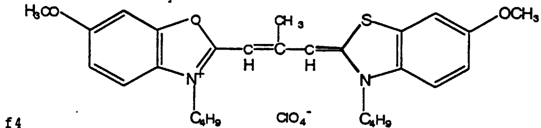
[Chemical Formula 224]
