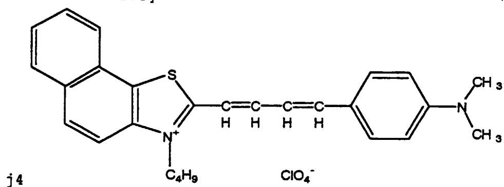
[Chemical Formula 251]
