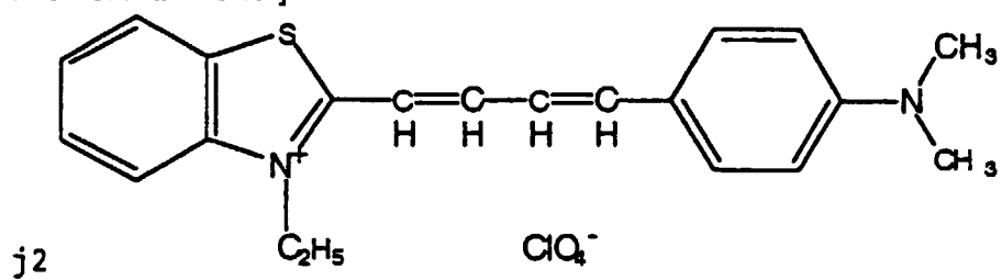
[Chemical Formula 249]
