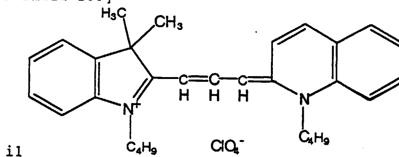
[Chemical Formula 235]
