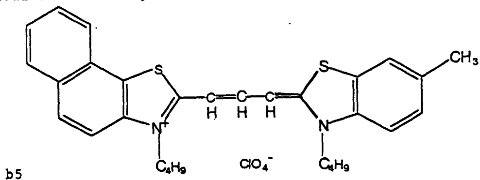
[Chemical Formula 203]
