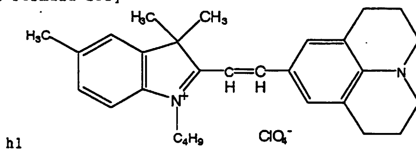
[Chemical Formula 231]
