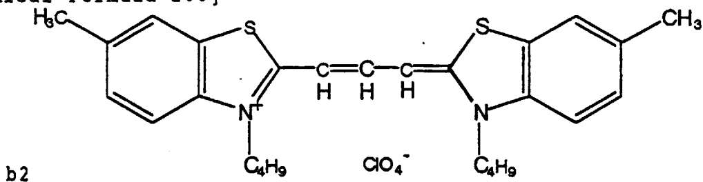
[Chemical Formula 200]
