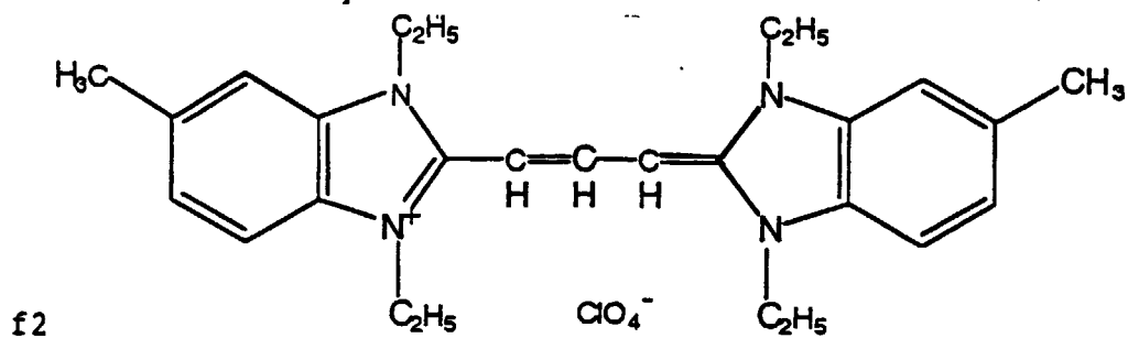
[Chemical Formula 222]
