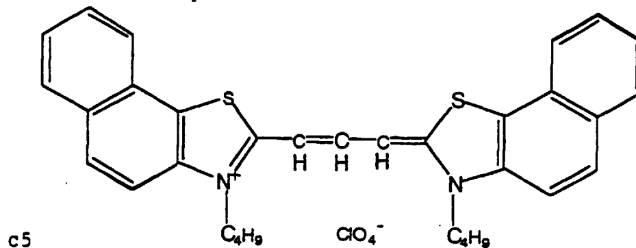
[Chemical Formula 211]
