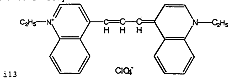
[Chemical Formula 247]
