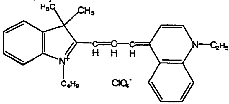
[Chemical Formula 243]
