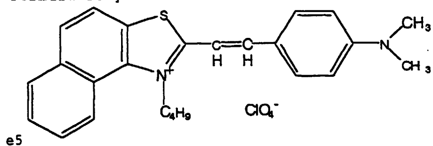
[Chemical Formula 220]
