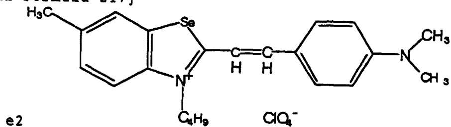
[Chemical Formula 217]
