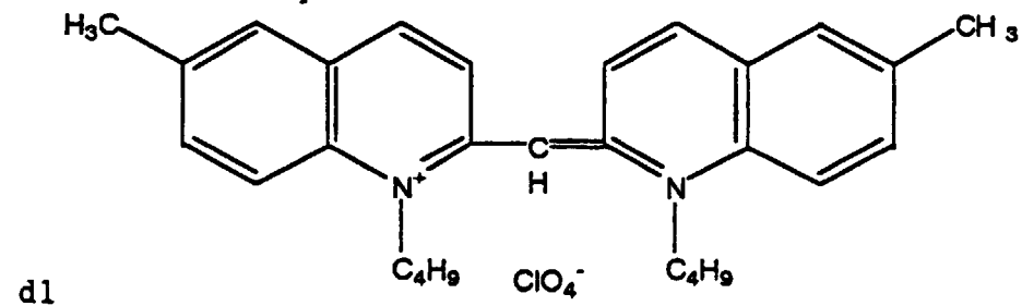
[Chemical Formula 214]
