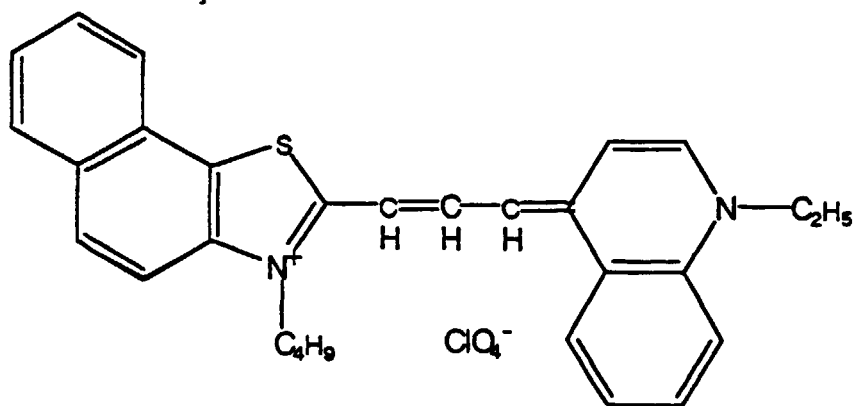
[Chemical Formula 246]
