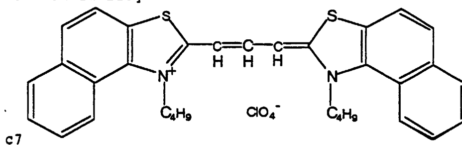
[Chemical Formula 213]
