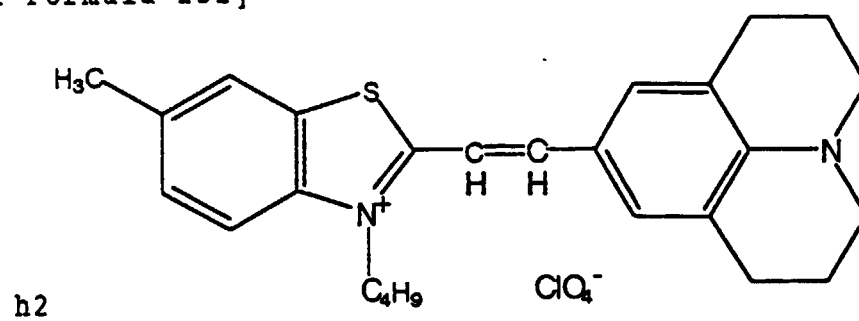
[Chemical Formula 232]
