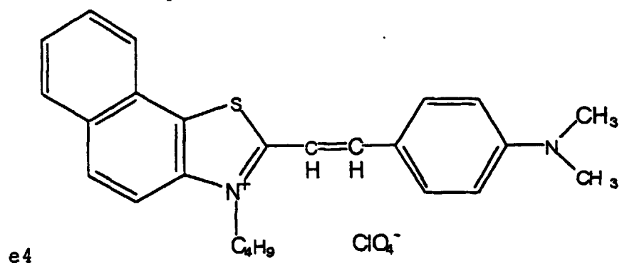
[Chemical Formula 219]
