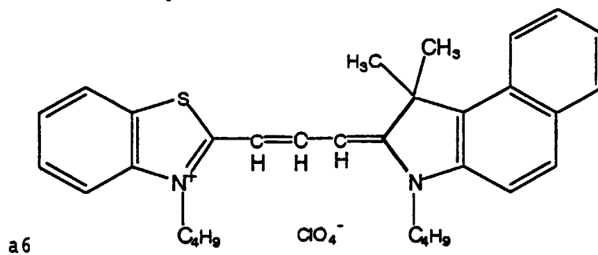
[Chemical Formula 196]
