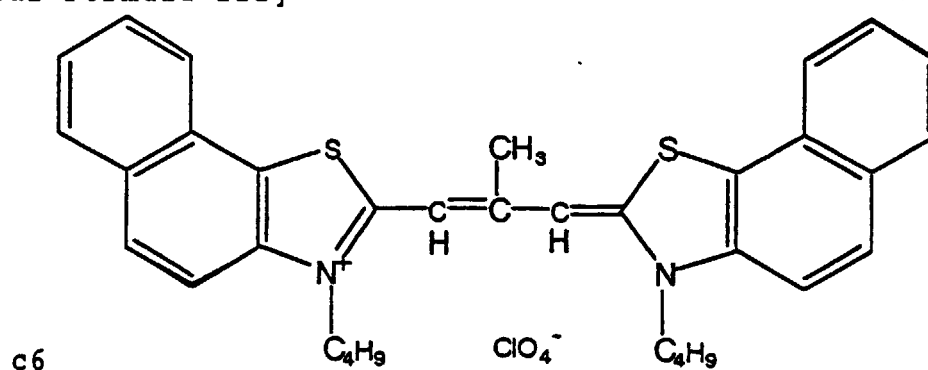
[Chemical Formula 212]
