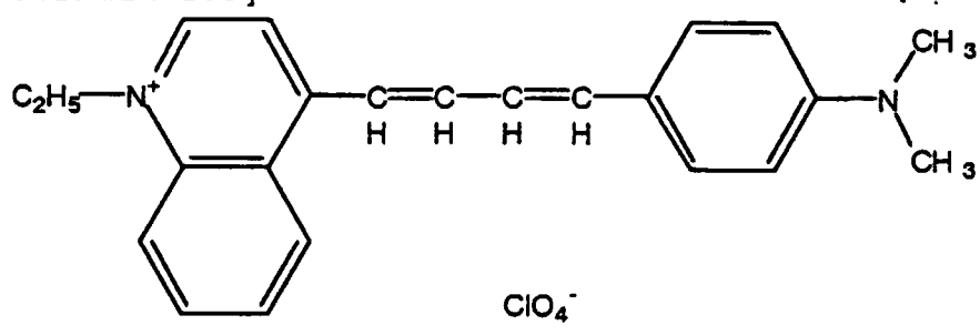
[Chemical Formula 253]
