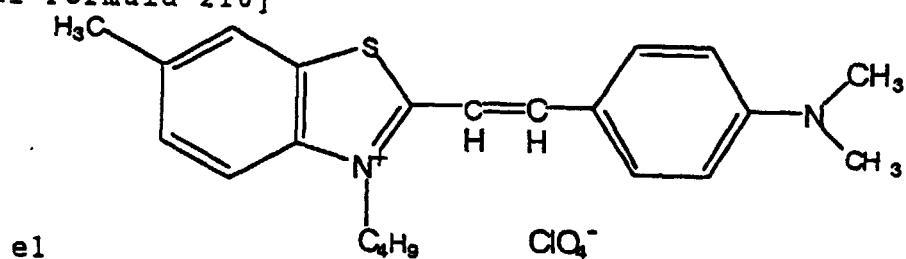
[Chemical Formula 216]
