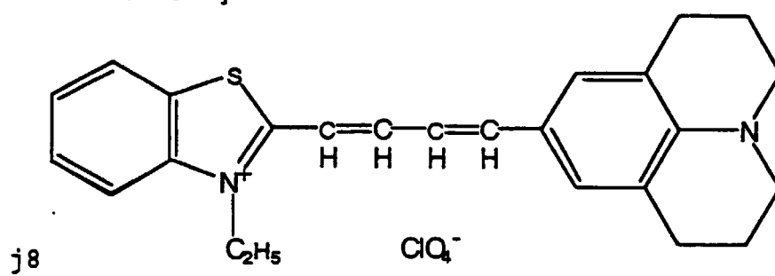
[Chemical Formula 255]
