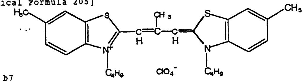
[Chemical Formula 205]
