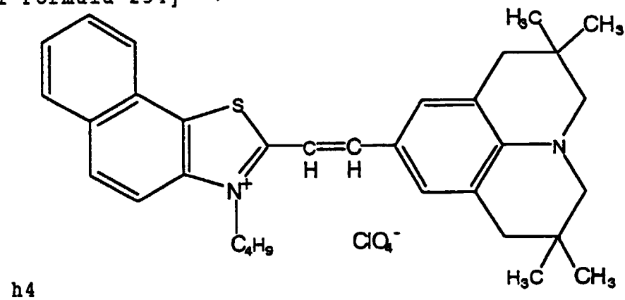
[Chemical Formula 234]
