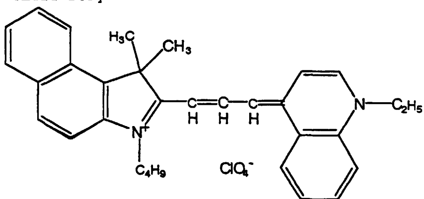
[Chemical Formula 245]
