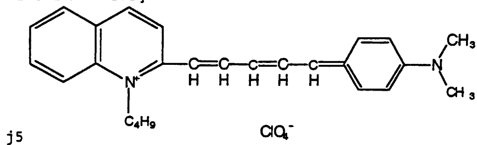
[Chemical Formula 252]
