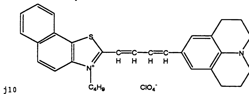
[Chemical Formula 257]
