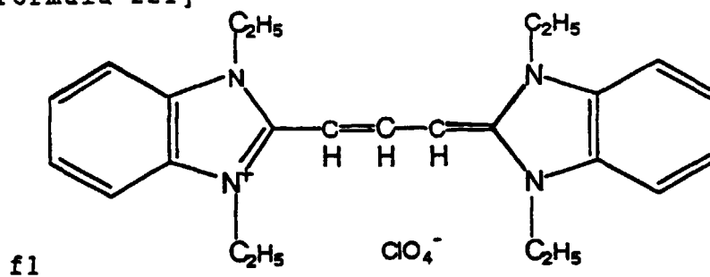
[Chemical Formula 221]
