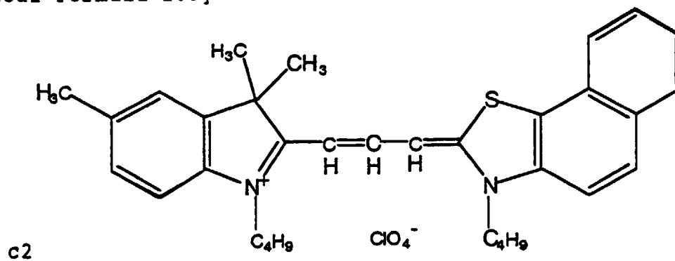
[Chemical Formula 208]
