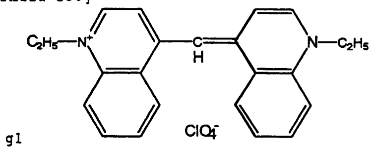
[Chemical Formula 230]
