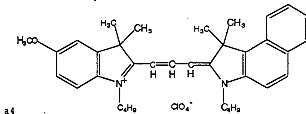
[Chemical Formula 194]
