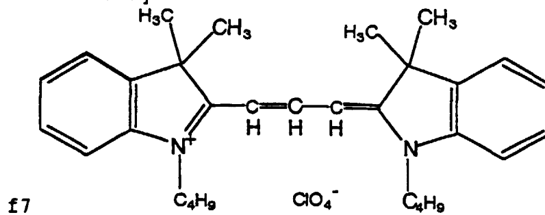
[Chemical Formula 227]
