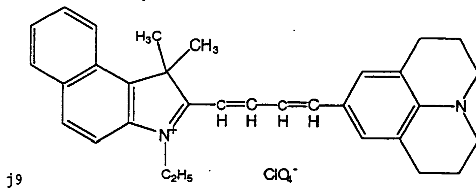
[Chemical Formula 256]
