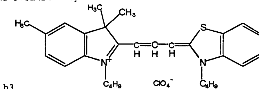
[Chemical Formula 201]
