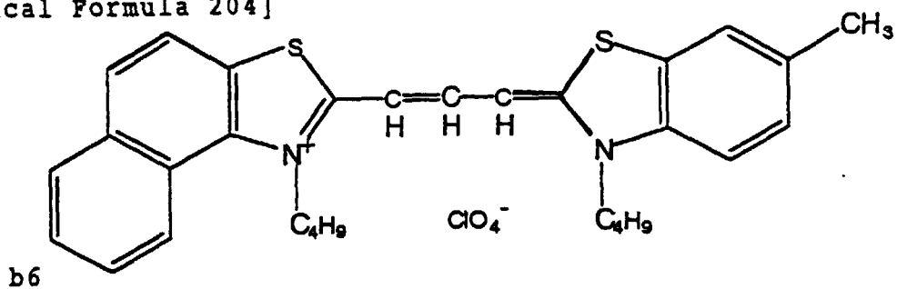
[Chemical Formula 204]
