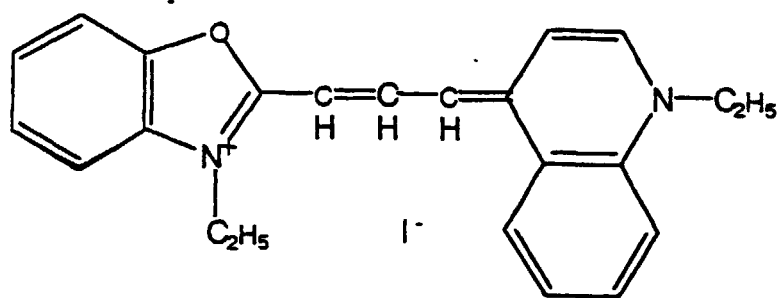
[Chemical Formula 241]
