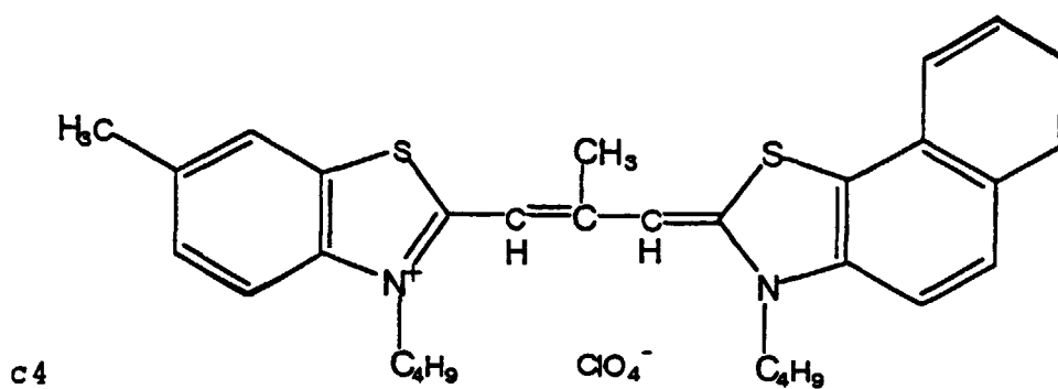
[Chemical Formula 210]
