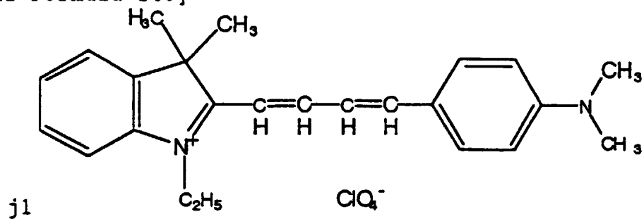
[Chemical Formula 248]
