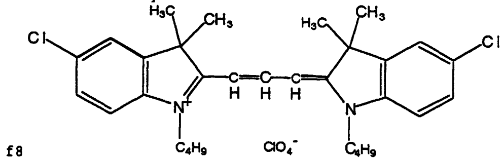
[Chemical Formula 228]
