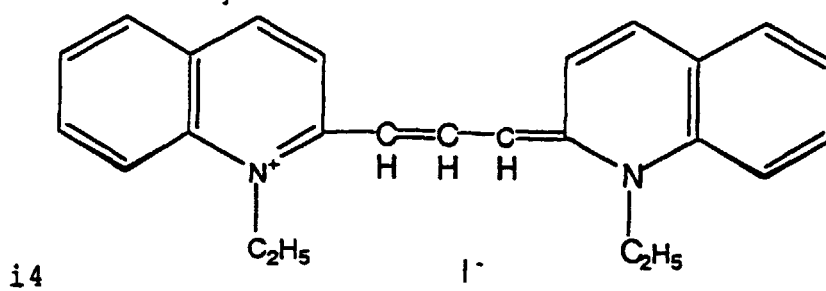
[Chemical Formula 238]
