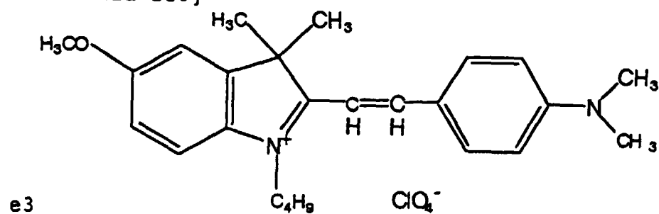
[Chemical Formula 218]
