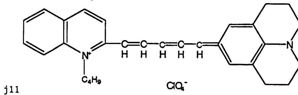
[Chemical Formula 258]
