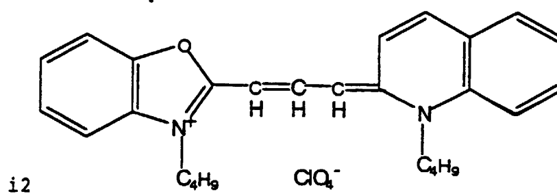
[Chemical Formula 236]
