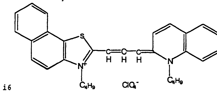
[Chemical Formula 240]
