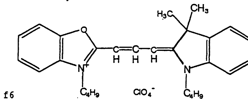
[Chemical Formula 226]
