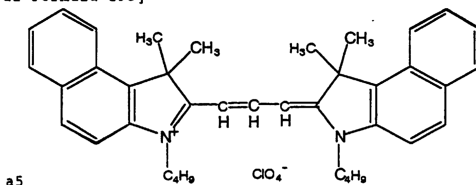
[Chemical Formula 195]
