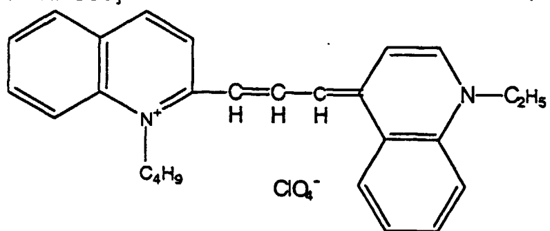
[Chemical Formula 244]
