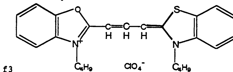
[Chemical Formula 223]
