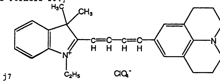
[Chemical Formula 254]
