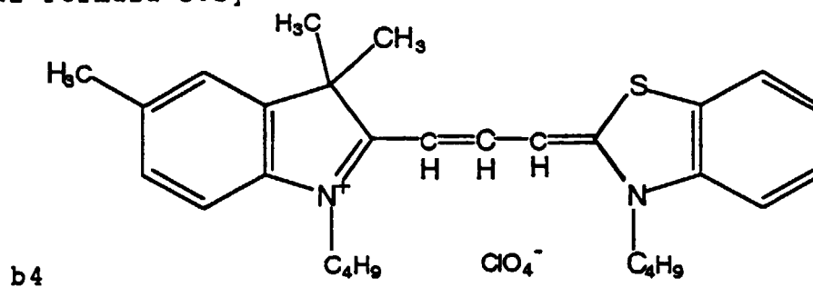
[Chemical Formula 202]
