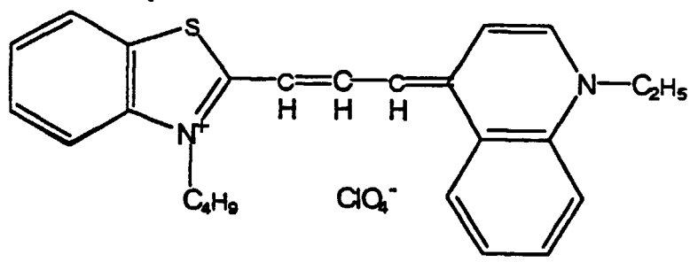
[Chemical Formula 242]
