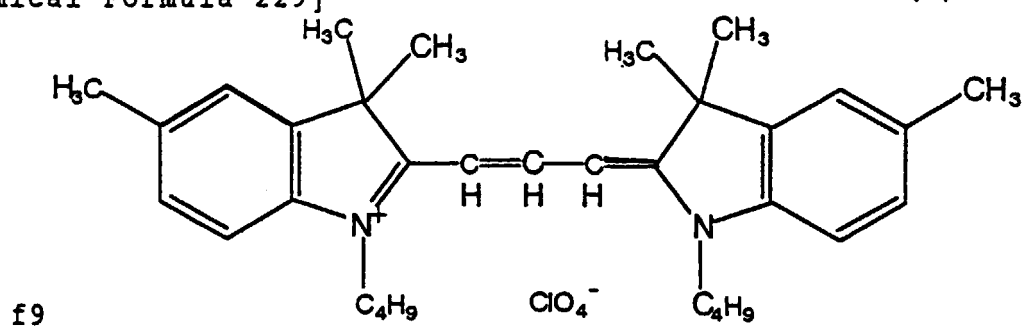
[Chemical Formula 229]
