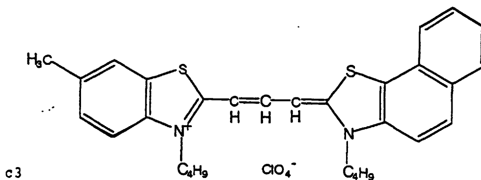
[Chemical Formula 209]
