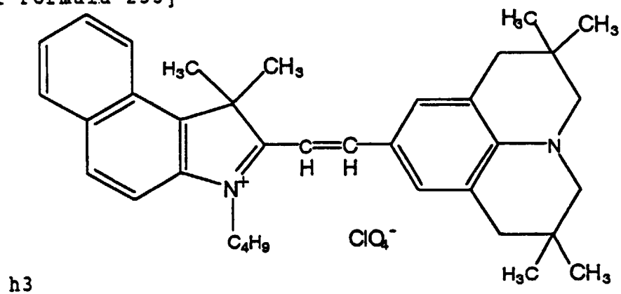
[Chemical Formula 233]
