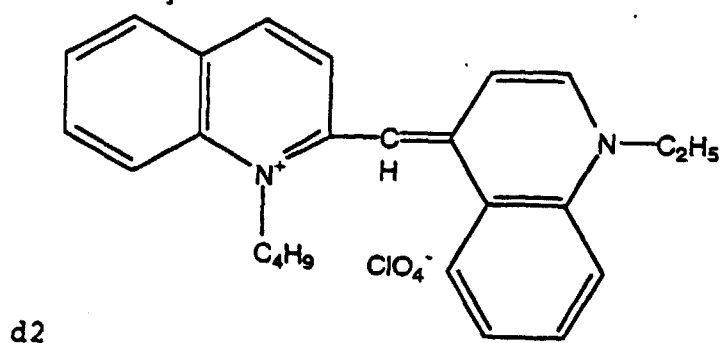
[Chemical Formula 215]
