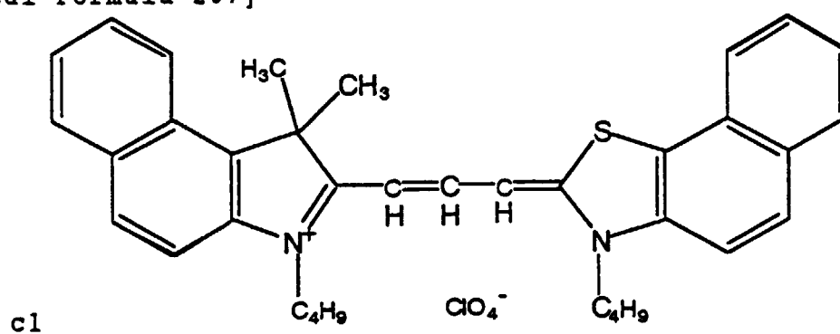
[Chemical Formula 207]
