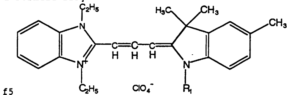
[Chemical Formula 225]
