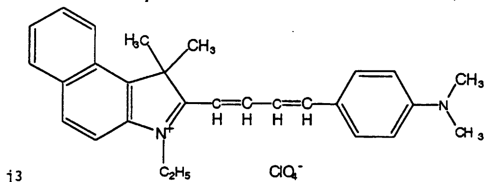
[Chemical Formula 250]
