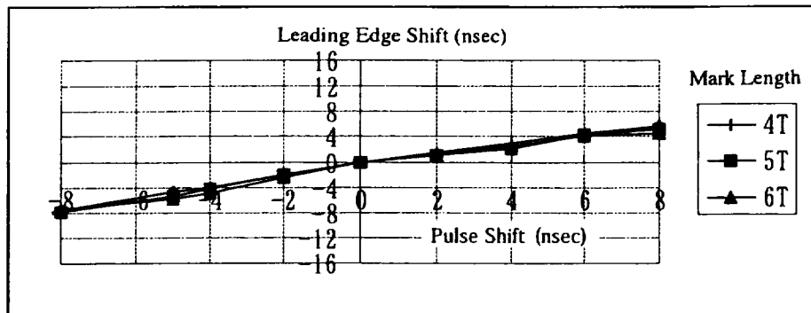
Leading Edge Shift with Leading Pulse Shift
