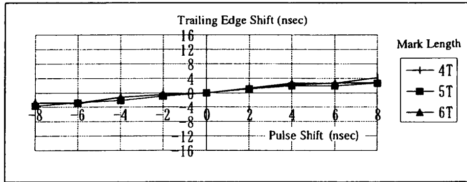
Trailing Edge Shift with Trailing Pulse Shift
