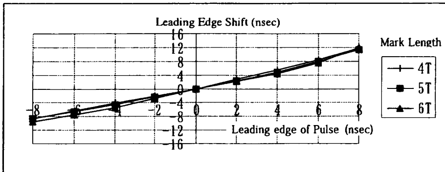
Leading Edge Shift with Variable Leading Edge of Pulse, and with Fixed Trailing Edge of Pulse
