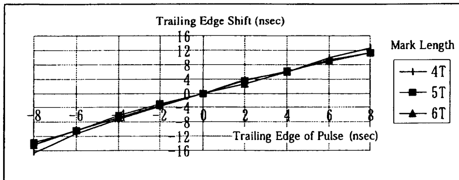
Trailing Edge Shift with valuable Trailing Edge of Pulse, and with fixed Leading Edge of Pulse
