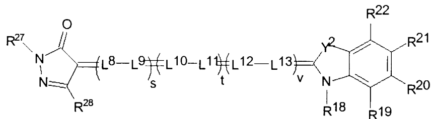
VIII-E
