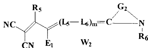
IIc
