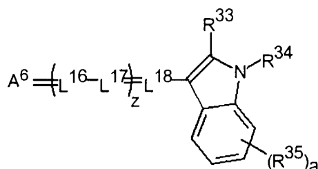
Formula X
