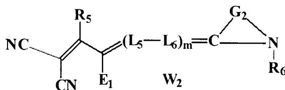
IIc
