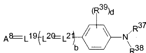
Formula XII
