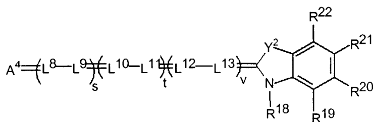
Formula VII-A
