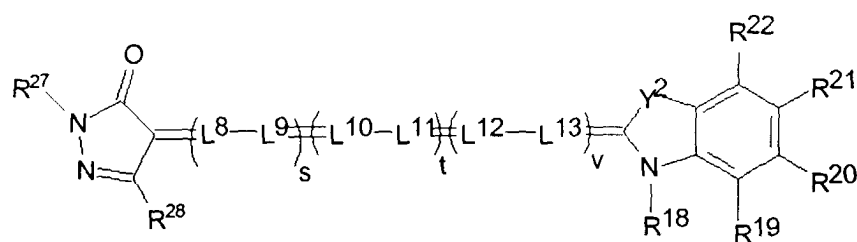
VIII-E
