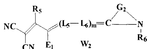
IIc
