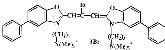
Dye D-1
