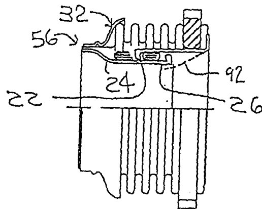
ASSEMBLE & SIZE END CAP FIG. 17
