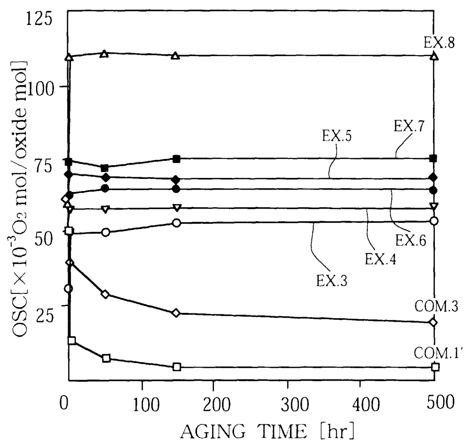
FIG.7 OSC IN REDUCING ATMOSPHERE
