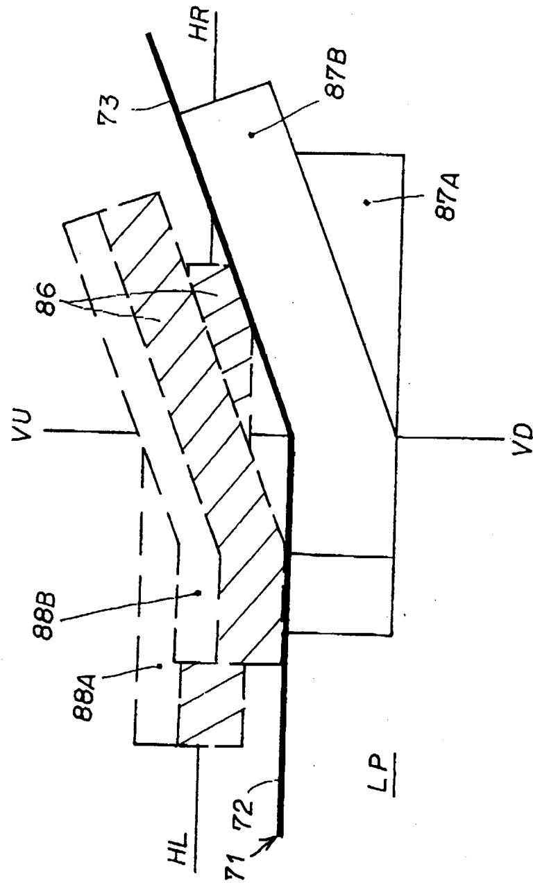
FIG. 23 PRIOR ART
