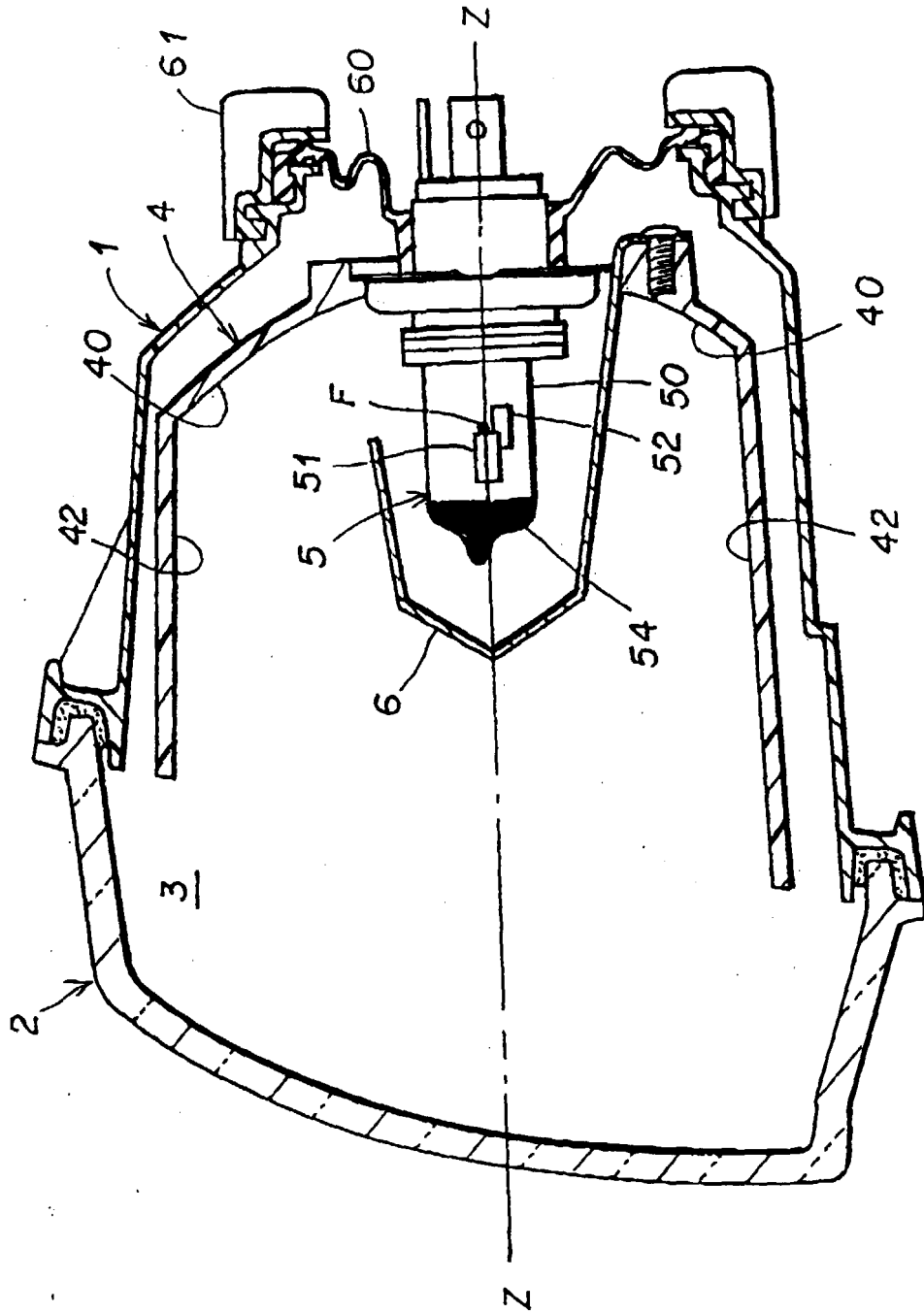
FIG.17 PRIOR ART
