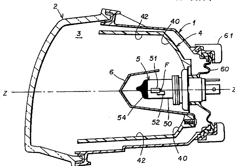
FIG.17 PRIOR ART
