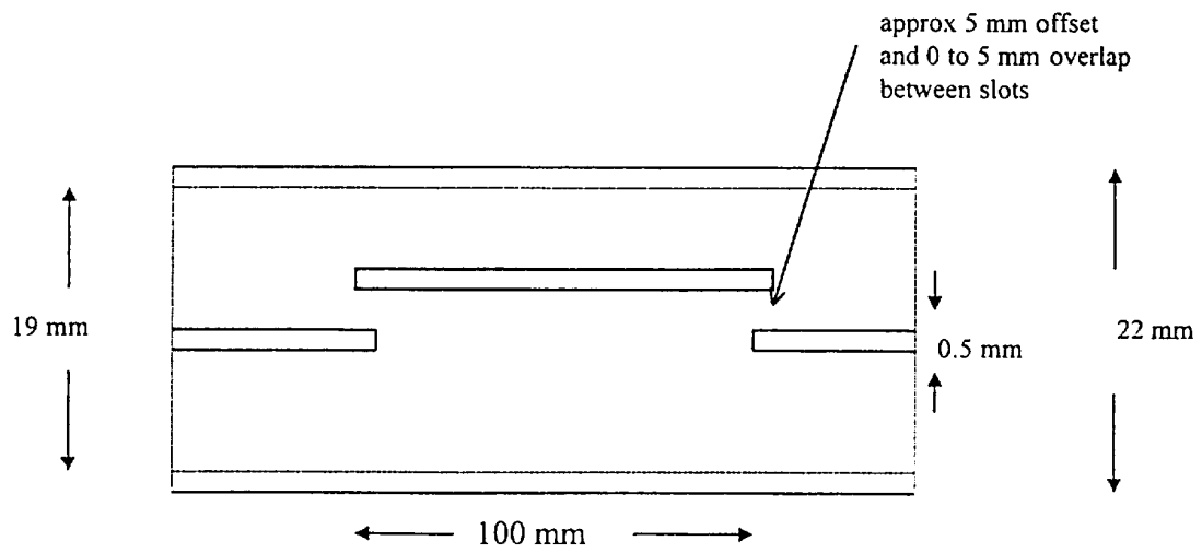
Typical slot size and arrangement
