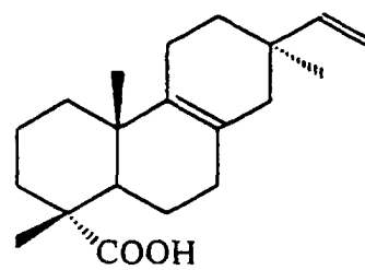
\Delta^8 -Pimaric 11
