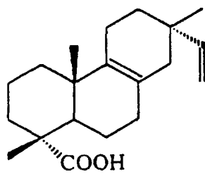
\Delta^8 -Isopimaric 9
