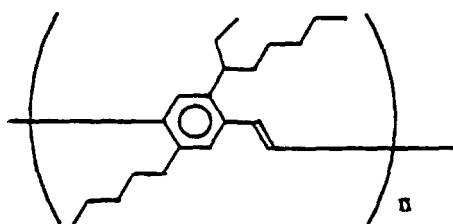
BuEH-PPV
