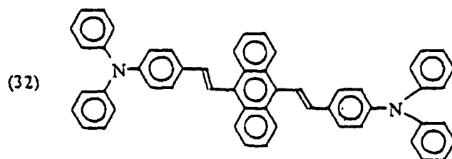
BSA
