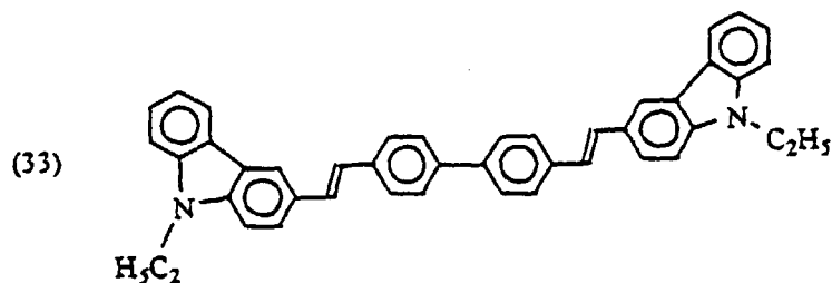
BCzVBi
