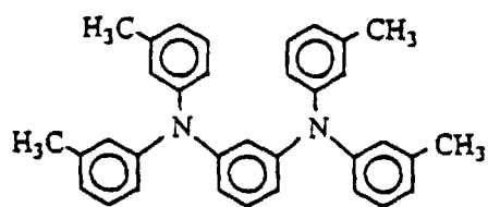
PDA
