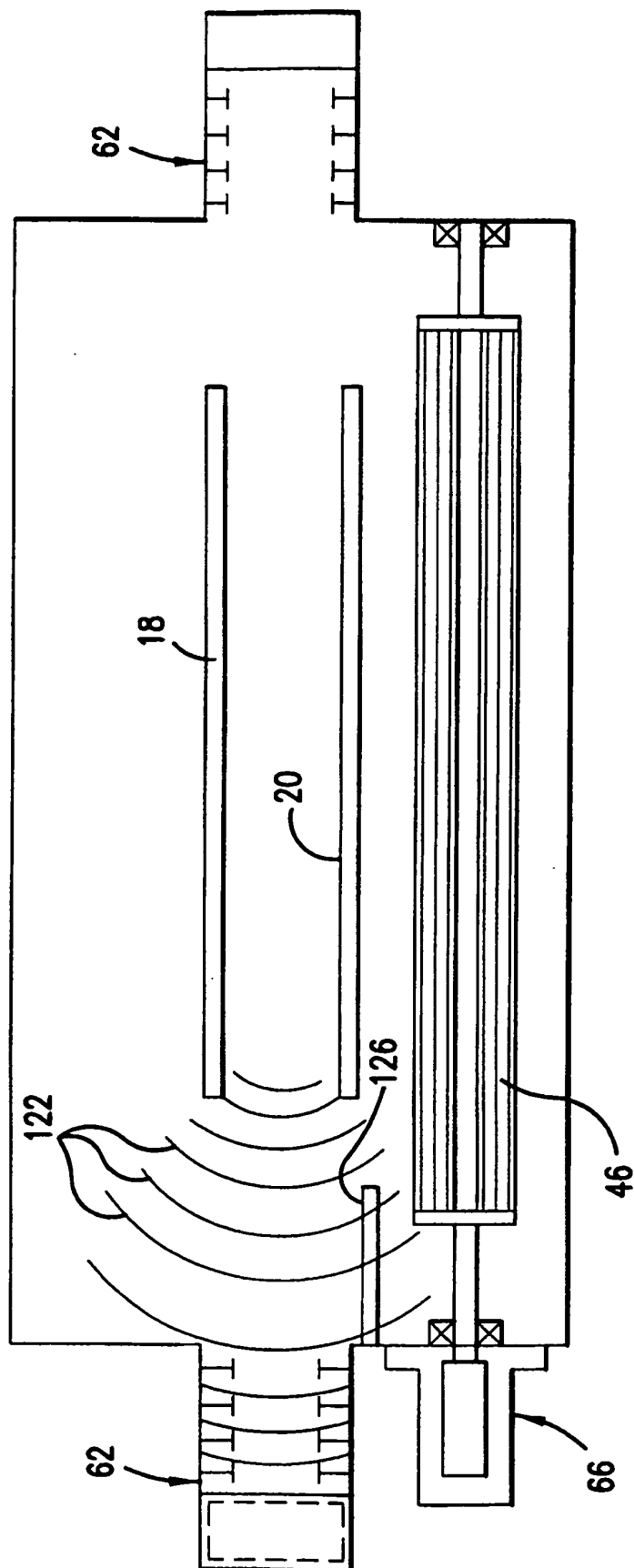
FIG. 2 PRIOR ART
