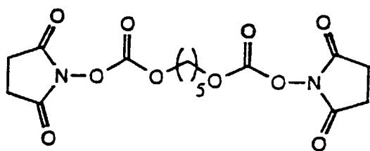
1,5-Bis(succinimidooxycarbonyloxy)pentane
