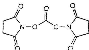
Di(succinimidyl) carbonate
