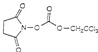
Succinimidyl-2,2,2-trichloroethyl Carbonate
