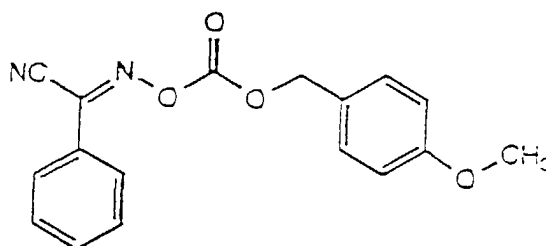
2-(4-methoxybenzyloxycarbonyloxyimino)-2-phenylacetonitrile
