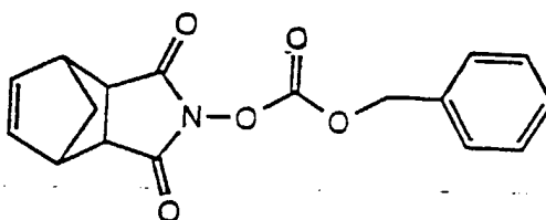
N-Benzyloxycarbonyloxy-5-norbornene-2,3-dicarboximide
