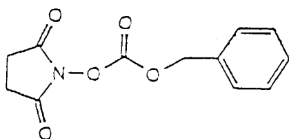
N-(Benzyloxycarbonyloxy)succinimide
