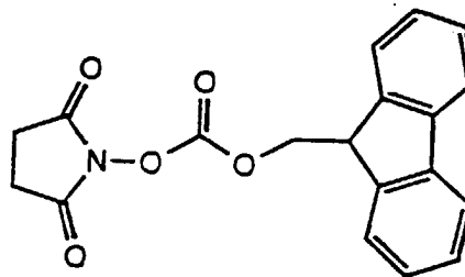
N-(9-fluorenylmethoxycarbonyloxy)succinimide
