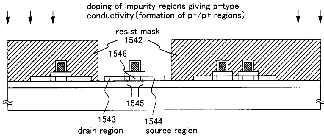
Fig. 17(B) 1545 : low concentration impurity region 1546 : channel forming region
