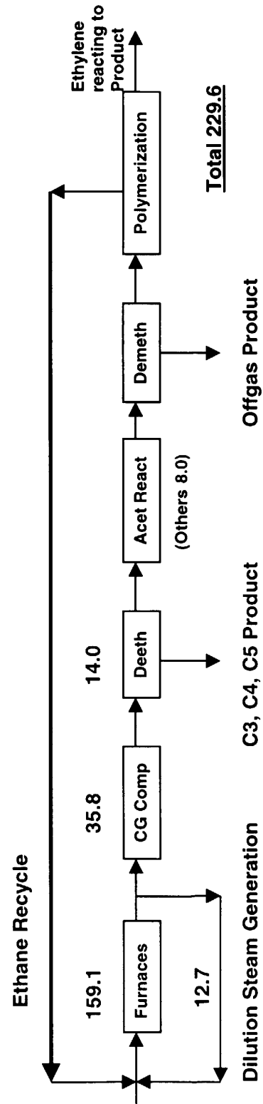
Figure 2b: New Process Heat Balance [GJ/hr.]
