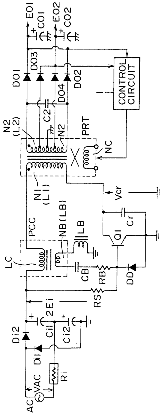
FIG. 10 (PRIOR ART)
