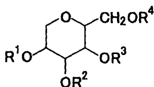
Formula (I-d)
