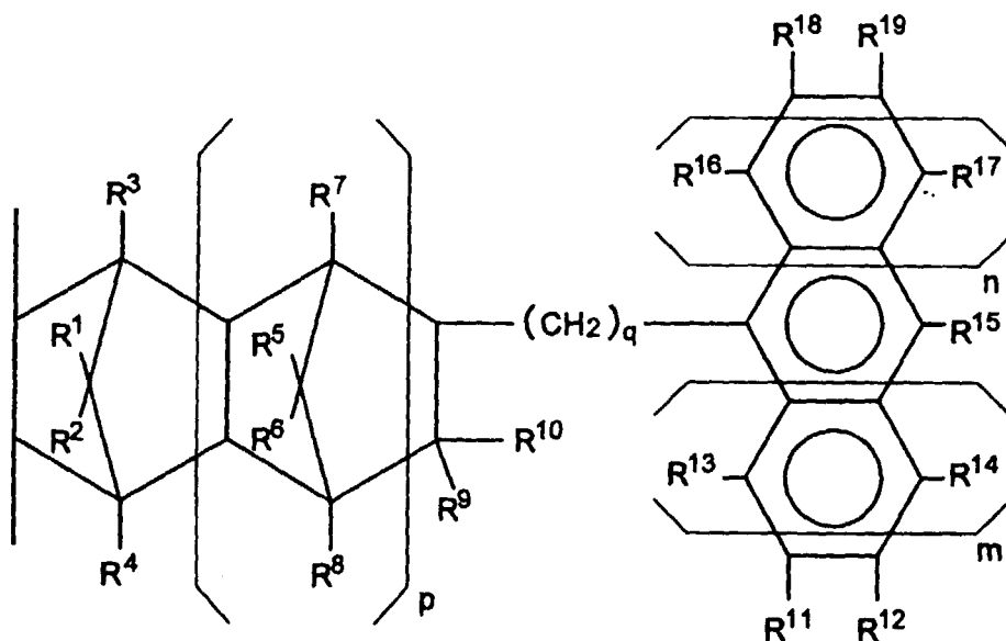
Formula (V)
