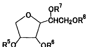
Formula (I-e)
