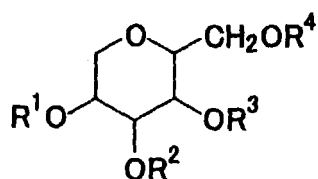
Formula (I-d)
