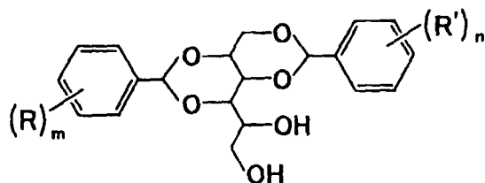
Formula (I-a)
