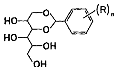
Formula (I-c)
