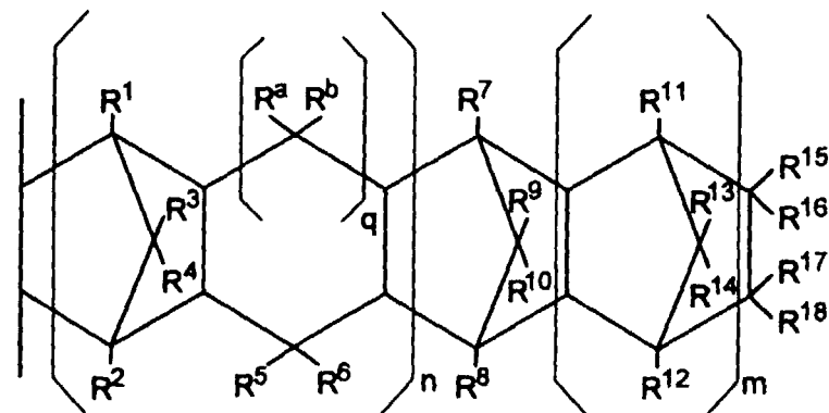
Formula (IV)
