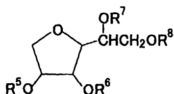
Formula (I-e)
