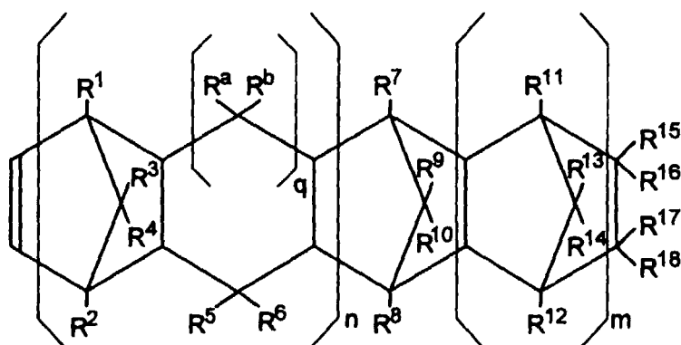
Formula (II)
