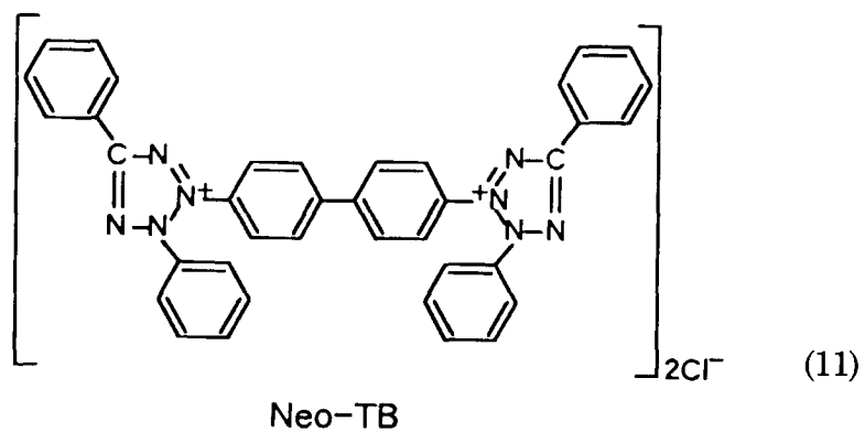
3,3'-(1,1'-biphenyl-4,4'-diyl)-bis(2,5-diphenyl)-2H-tetrazolium chloride
