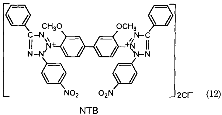
3,3'-(3,3'-dimethoxy-1,1'-biphenyl-4,4'-diyl)-bis[2-(4-nitrophenyl)-5-phenyl]-2H-tetrazolium chloride
