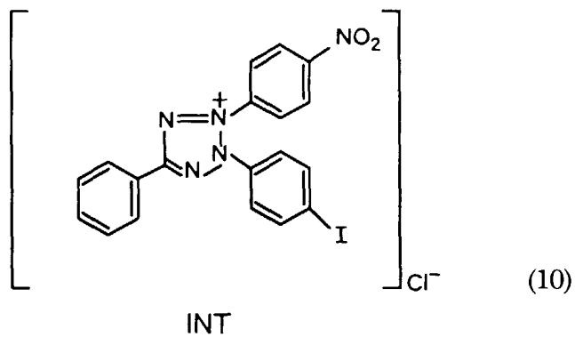
2-(4-iodophenyl)-3-(4-nitrophenyl)-5-phenyl-2H-tetrazolium chloride
