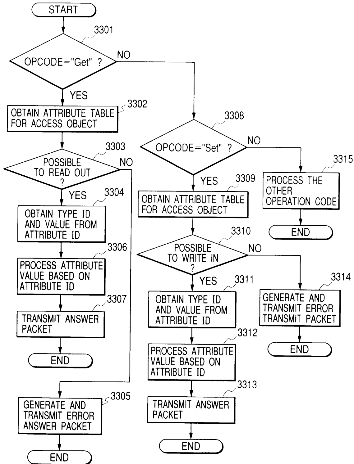
FLOW CHART OF ATTRIBUTE TABLE ACCESS
