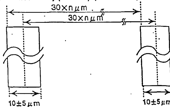
Fig. 5b Slit Dimension Accuracy (Precision) (at r=22.2mm)
