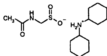
compound VII
