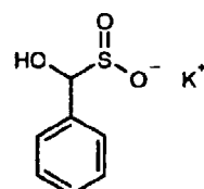
compound IV
