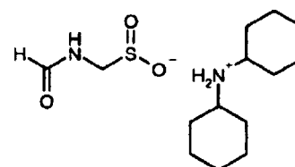
compound VI
