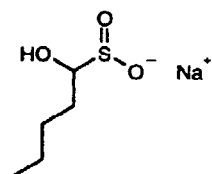
compound III
