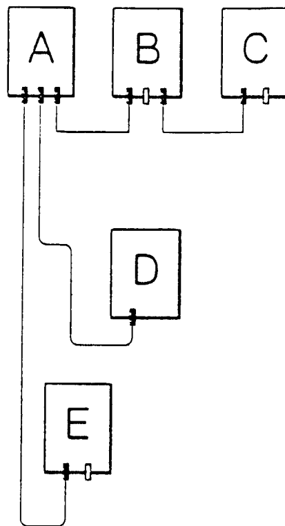
IEEE 1394 BUS CONNECTION
