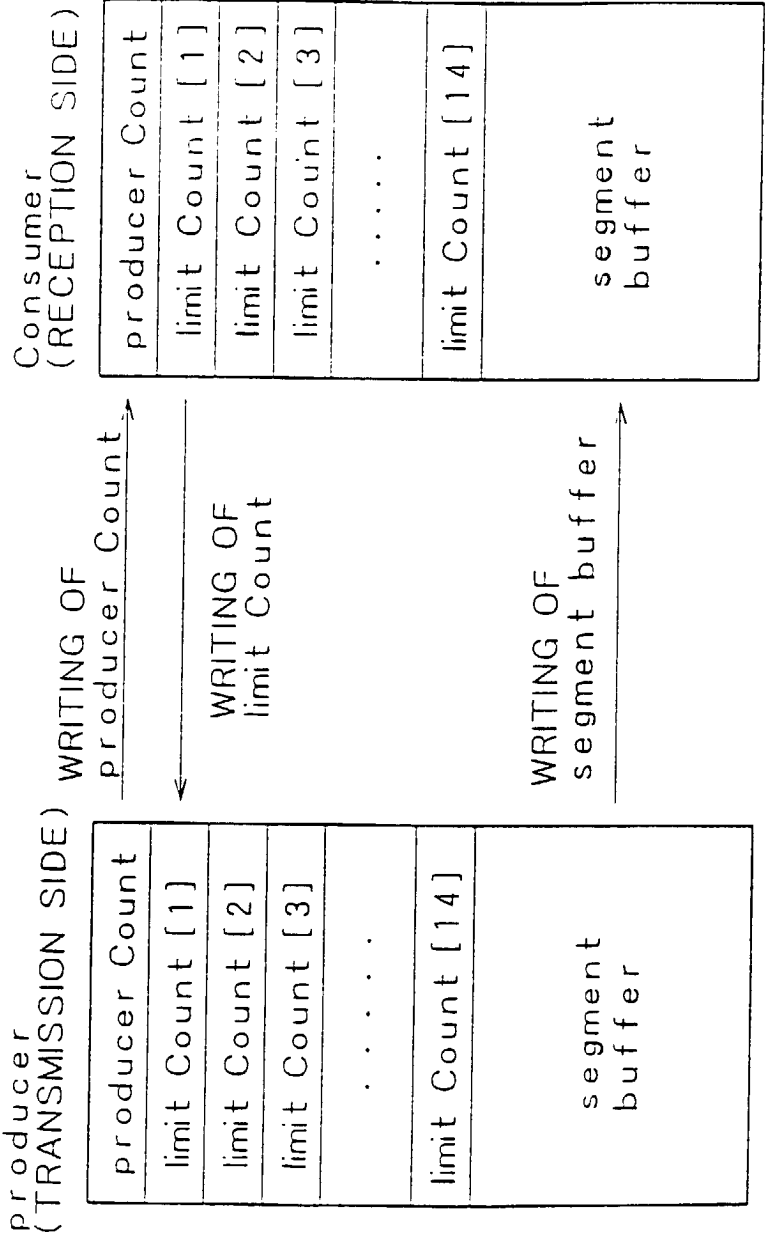
Asynchronous plug organization (2)
