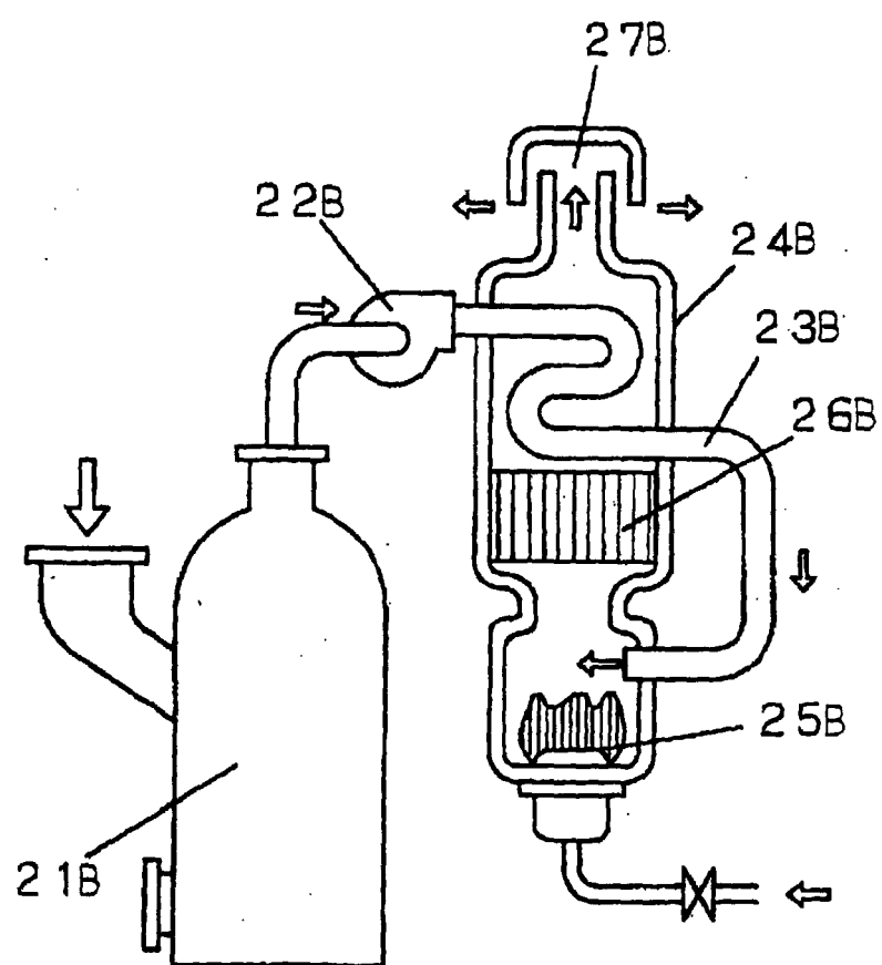
Fig. 19 PRIOR ART
