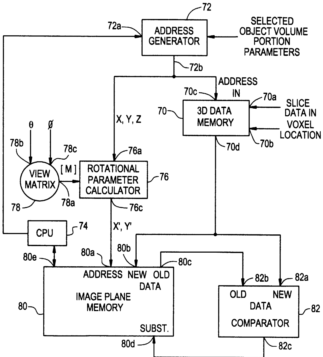
FIG.6 PRIOR ART
