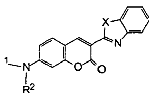
FD7 R = Me
