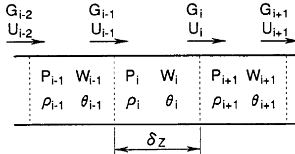
DISCRETE MODEL OF PIPE LINE
