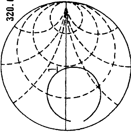
(a) Impedance characteristics
