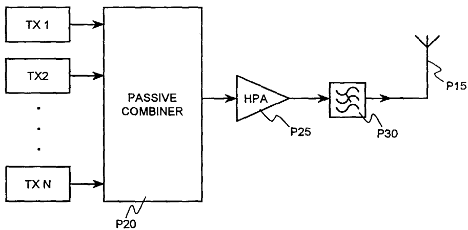
FIGURE 3 (PRIOR ART)
