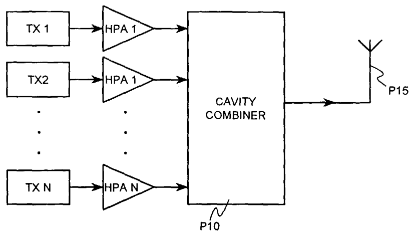
FIGURE 2 (PRIOR ART)
