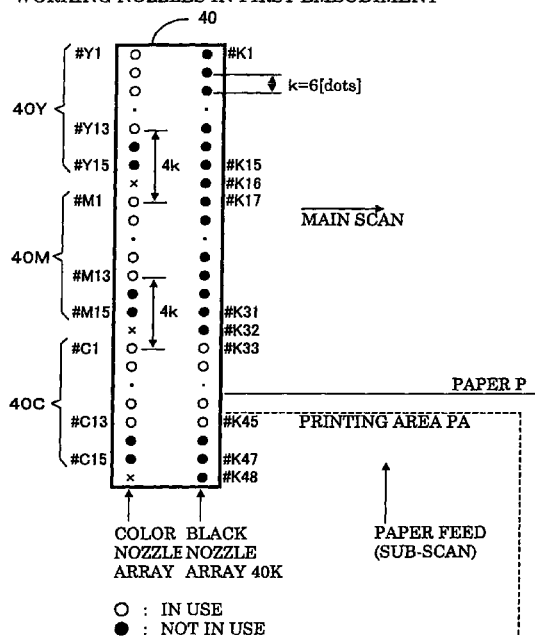
Fig. 7 WORKING NOZZLES IN FIRST EMBODIMENT
