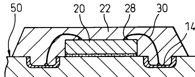
Fig. 2(c) PRIOR ART
