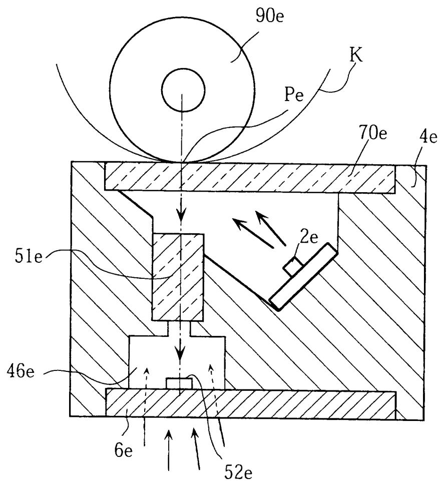
FIG.14 PRIOR ART
