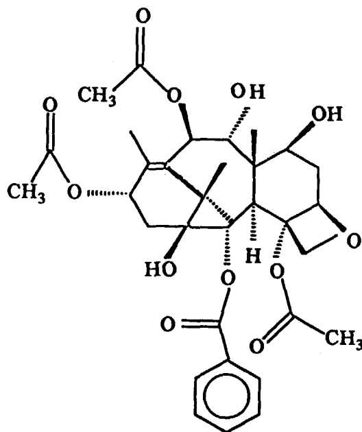
13-acetyl-9-dihydrobaccatin III
