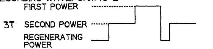
RECORDING WAVEFORM 15-2
