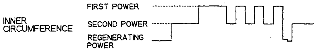
RECORDING WAVEFORM 17-2
