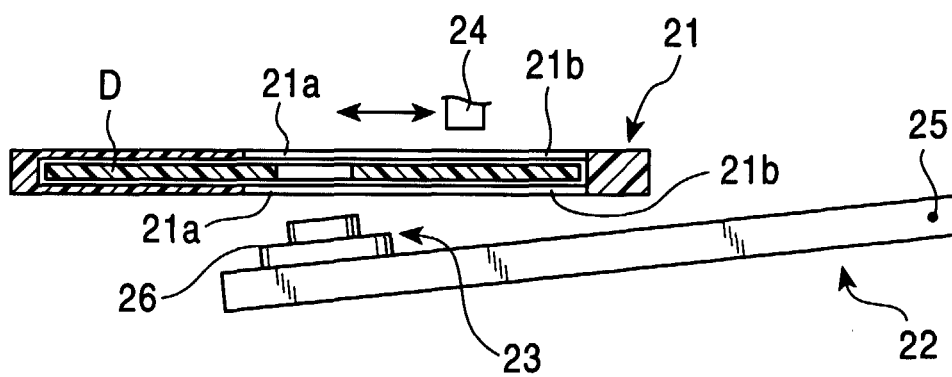
FIG. 31 PRIOR ART
