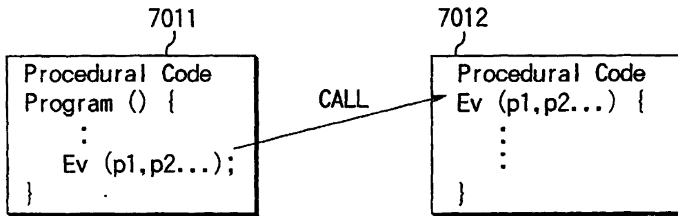
HANDLING OF EVENT BY ENGINE-1 SYSTEM
