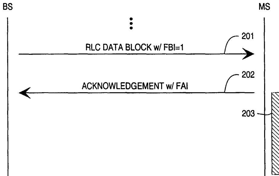
Fig. 2 PRIOR ART
