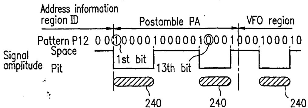
FIG. 24H Next state : 3 or 4, ID end : Space
