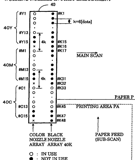
WORKING NOZZLES IN FIRST EMBODIMENT
