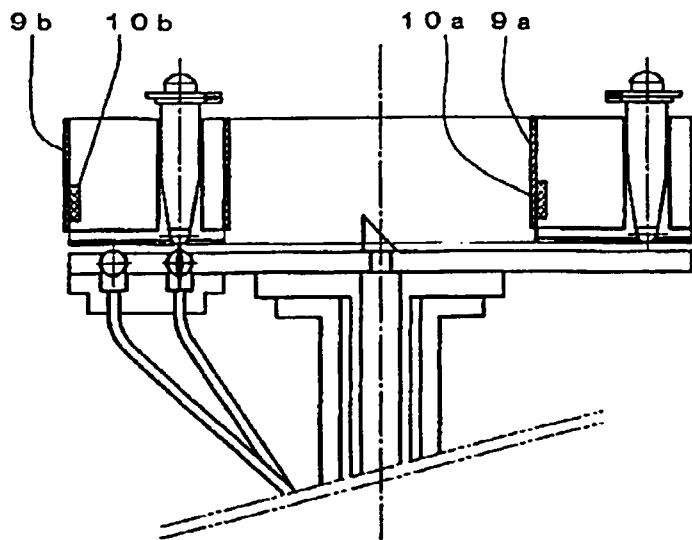
Enlarged view of temperature-controlling means (2 : 1)
