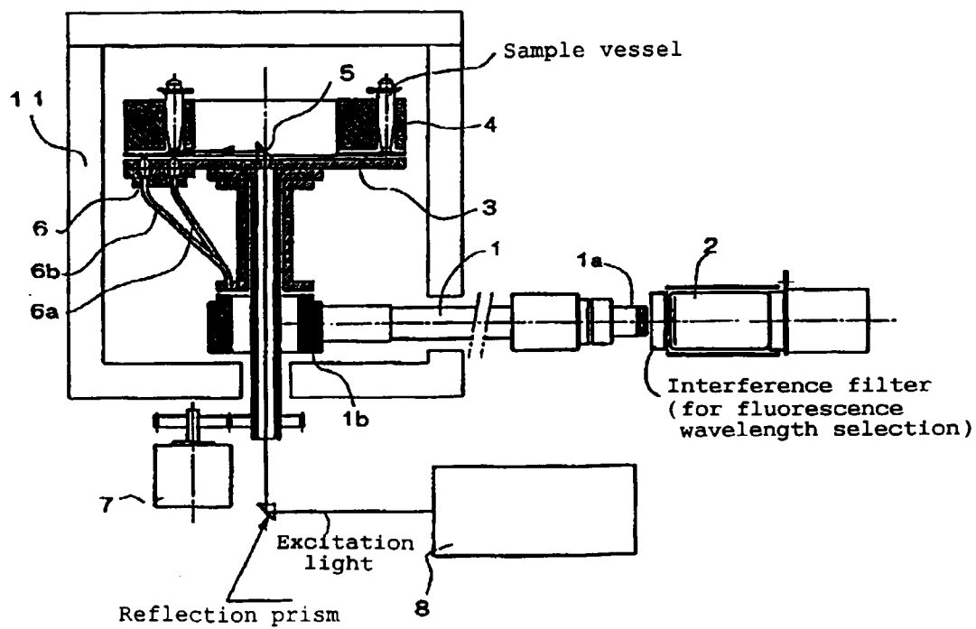
Front view (partially in cross section)
