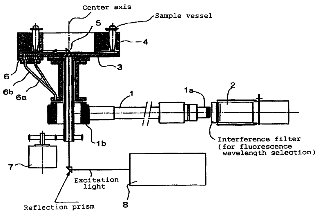
Front view (partially in cross section)
