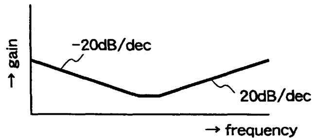
Fig.15 (b) gain characteristics of spot position loop filter 111
