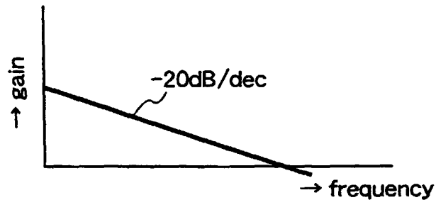
Fig.19 (b) gain characteristics of spot position loop filter 111
