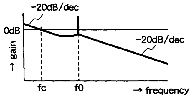
Fig.19 (e) open-loop characteristics of whole spot position control
