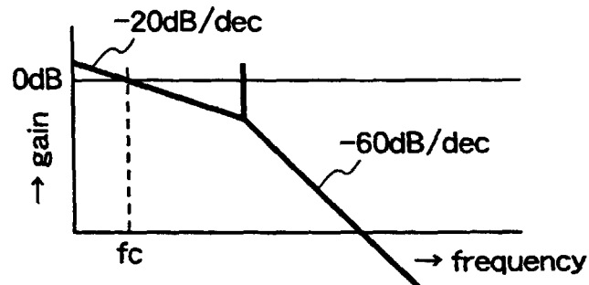
Fig.19 (c) open-loop characteristics of whole spot position control
