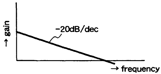
Fig.17 (b) gain characteristics of spot position loop filter 111
