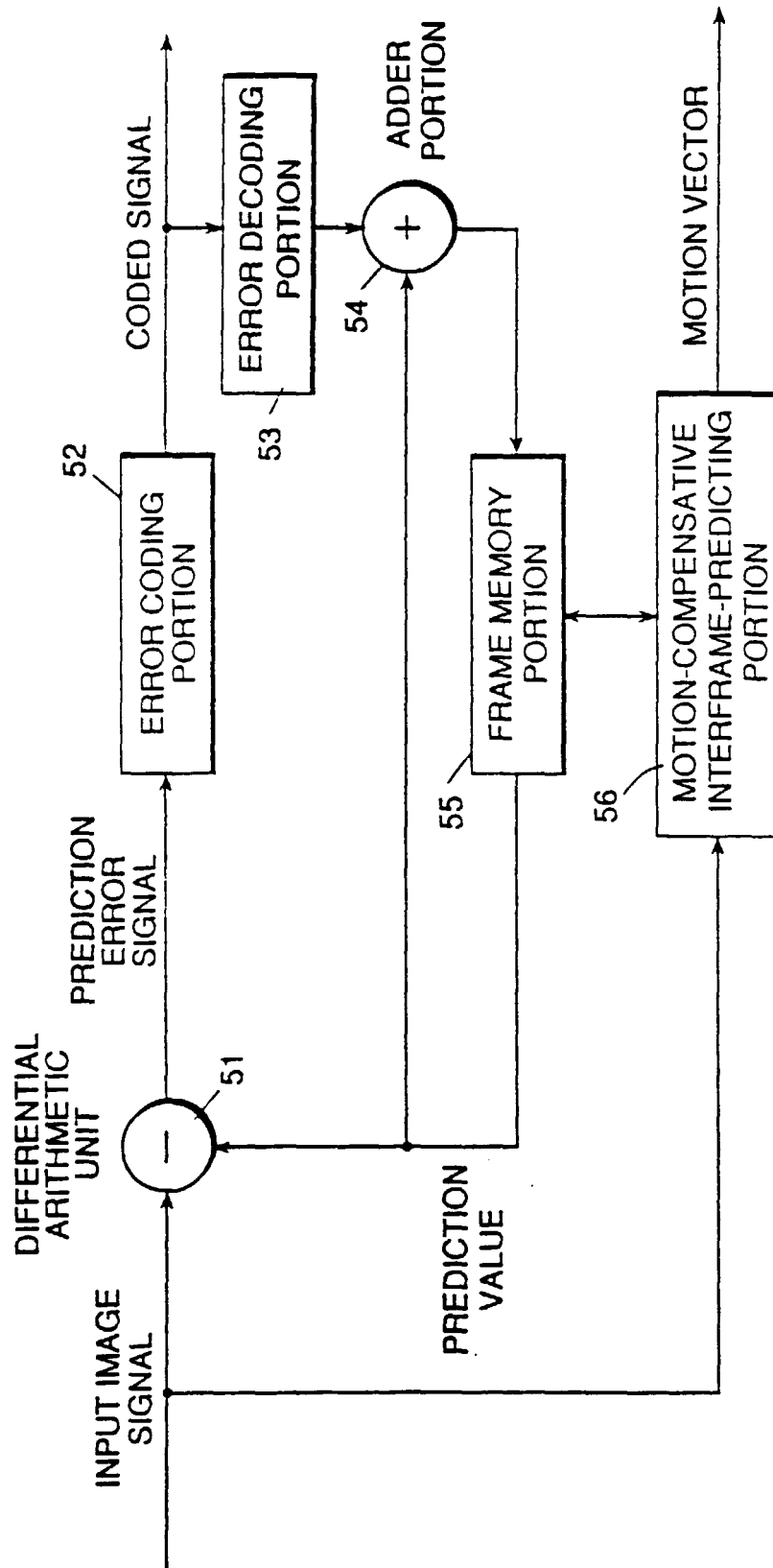
FIG.8 (PRIOR ART)
