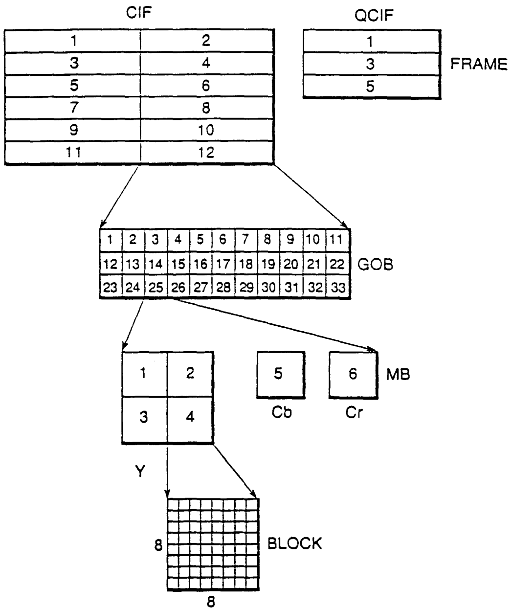
FIG.5 ( PRIOR ART )
