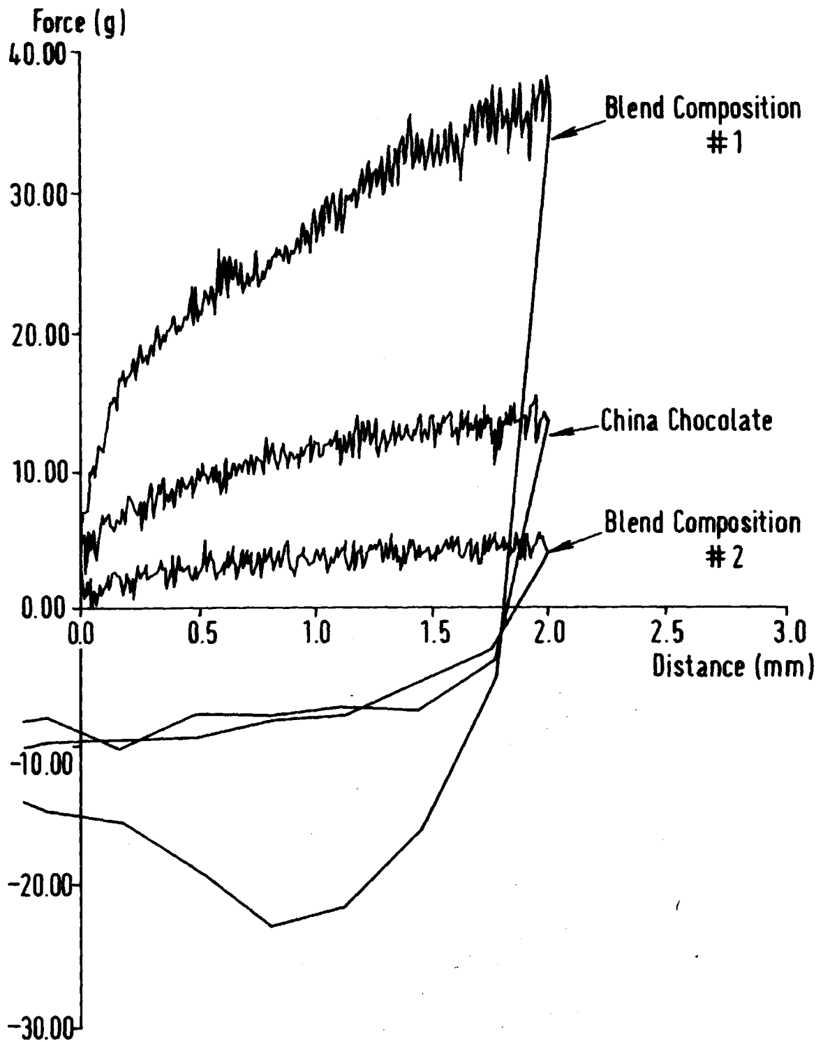
FIG.2 :TA-XT2 TEXTURE RESULTS AT 32°C
