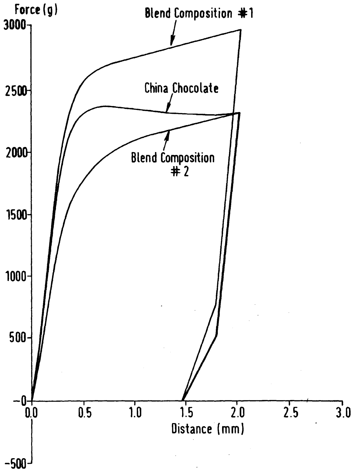
FIG.1: TA-XT2 TEXTURE RESULTS AT 20°C
