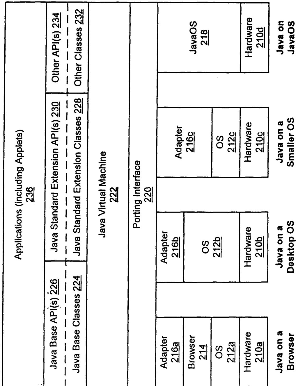
FIG. 2 (PRIOR ART)
