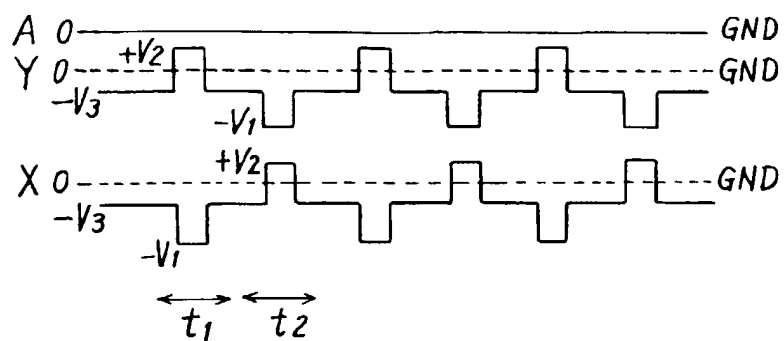
FIG. 6A Drive Wave Form
