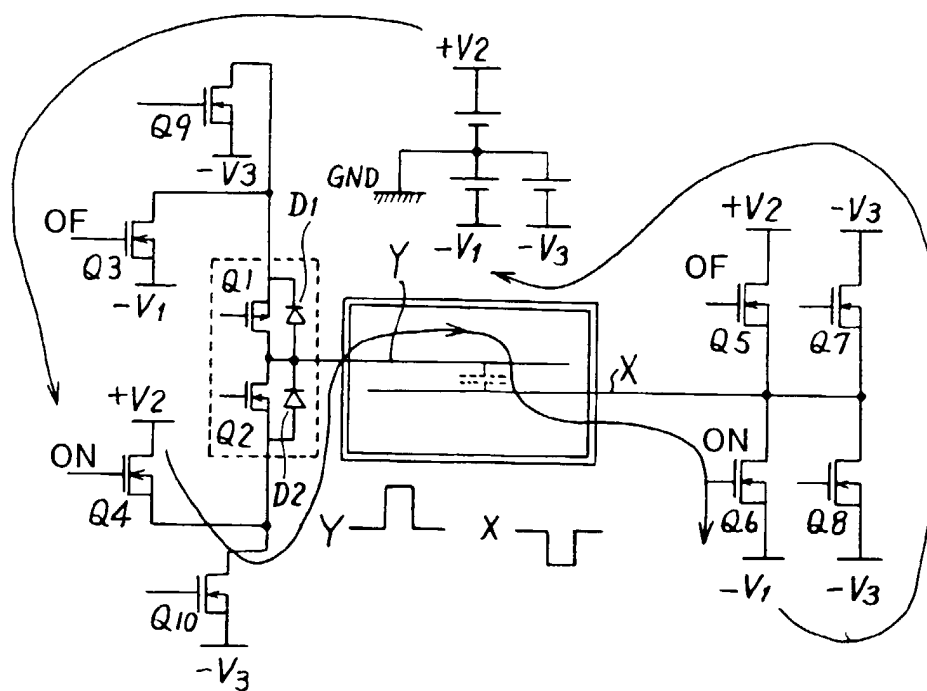
FIG. 6B Drive Circuit
