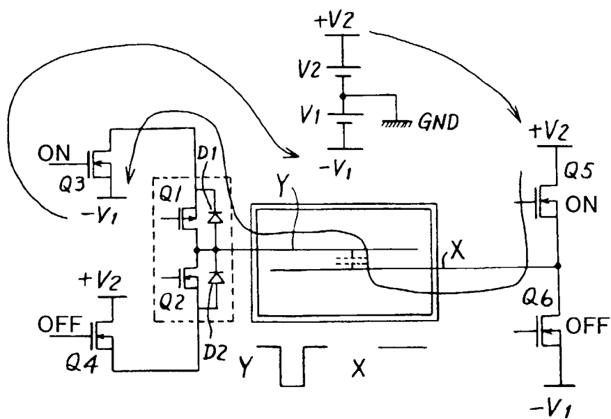
FIG. 5B Drive Circuit
