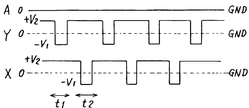
FIG. 5A Drive Wave Form
