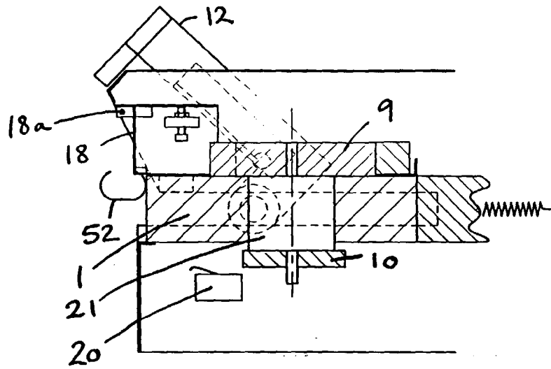
SECTION 'Z-Z'
